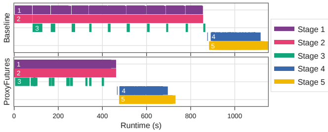
Fig. 8. 1000 Genomes Workflow stage start and ends times. ProxyFutures reduces workflow makespan by starting computations when data are available rather than when prior tasks complete.
