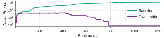
Fig. 10. Number of active proxies (i.e., proxies that still have a stored target object) during the runtime of the MOF Generation application. Our ownership model for proxies appropriately cleans up proxies when no longer needed while maintaining the benefits of the pass-by-reference model.
